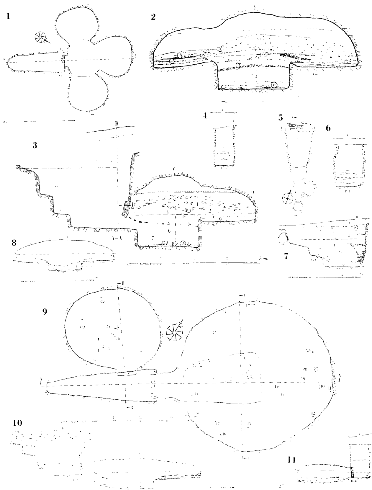
Fig. 126. Ajos Jakovos. Tomb 8, Plan (1); Sections C-C, A-A, B-B (2, 3, 4). Tomb 9, Plan (5); Sections B-B, A-A (6, 7). Tomb 10, Section C-C (8); Plan (9); Sections A-A, B-B (10, 11).
